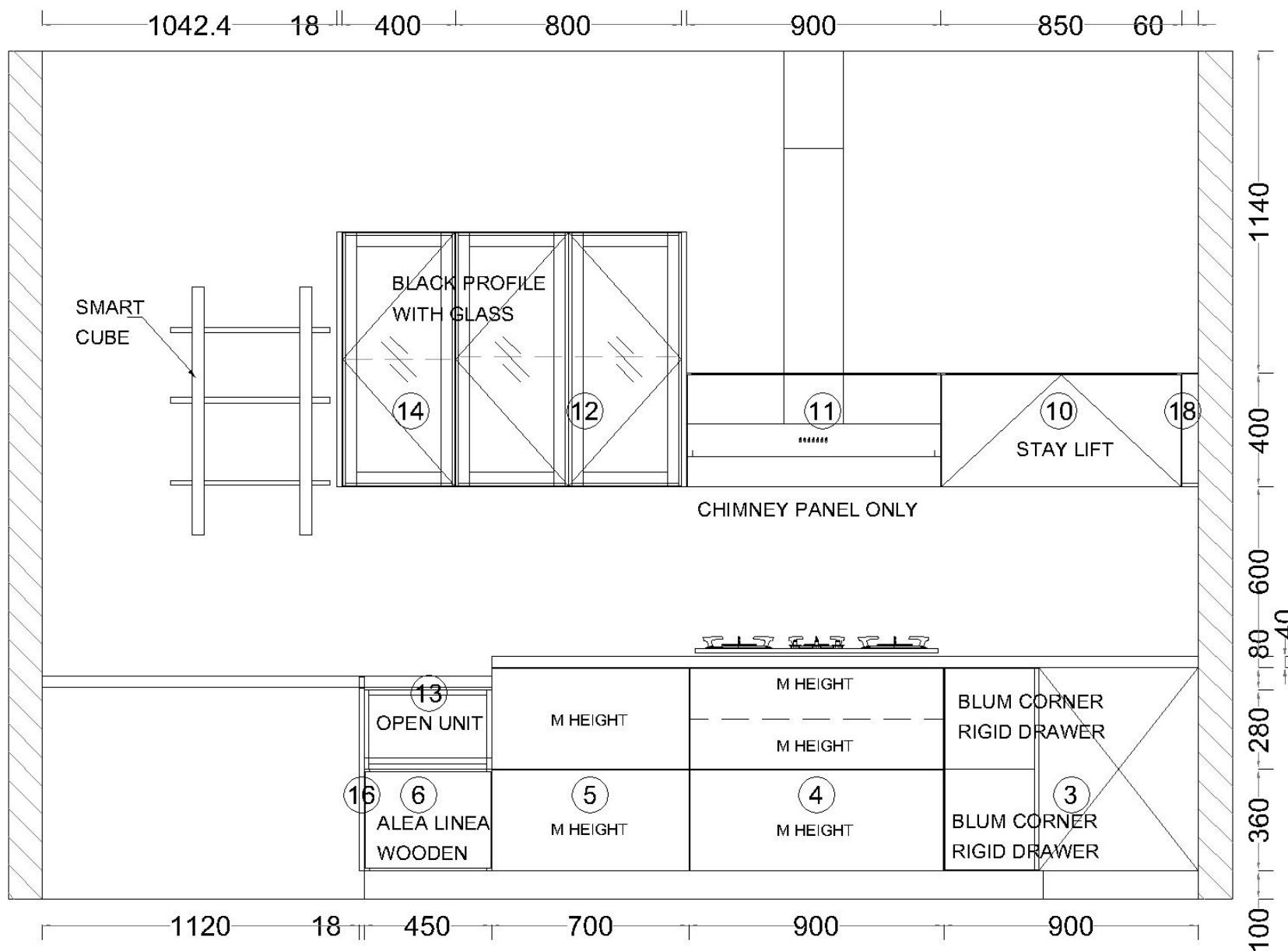
A View elevation drawing
