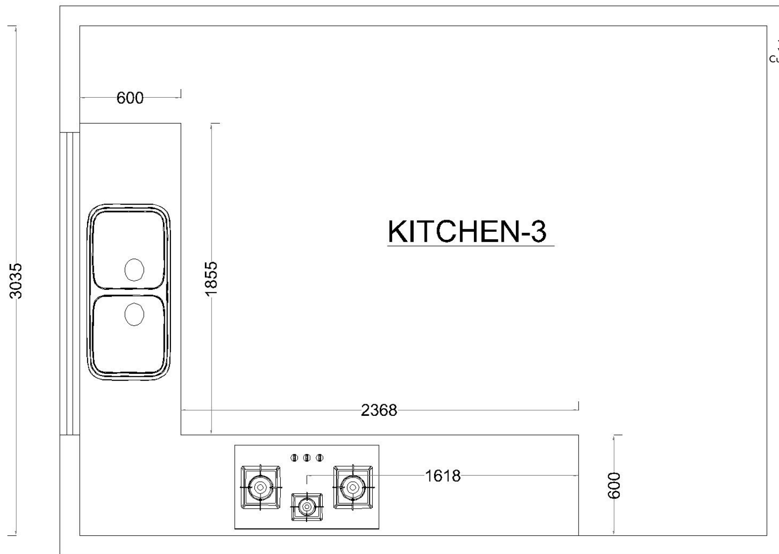
WORKTOP PLAN
