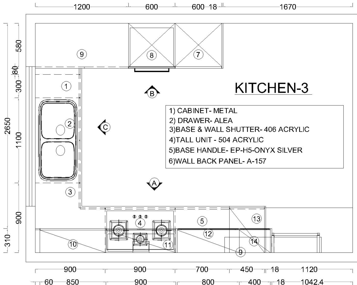
Plan drawing
