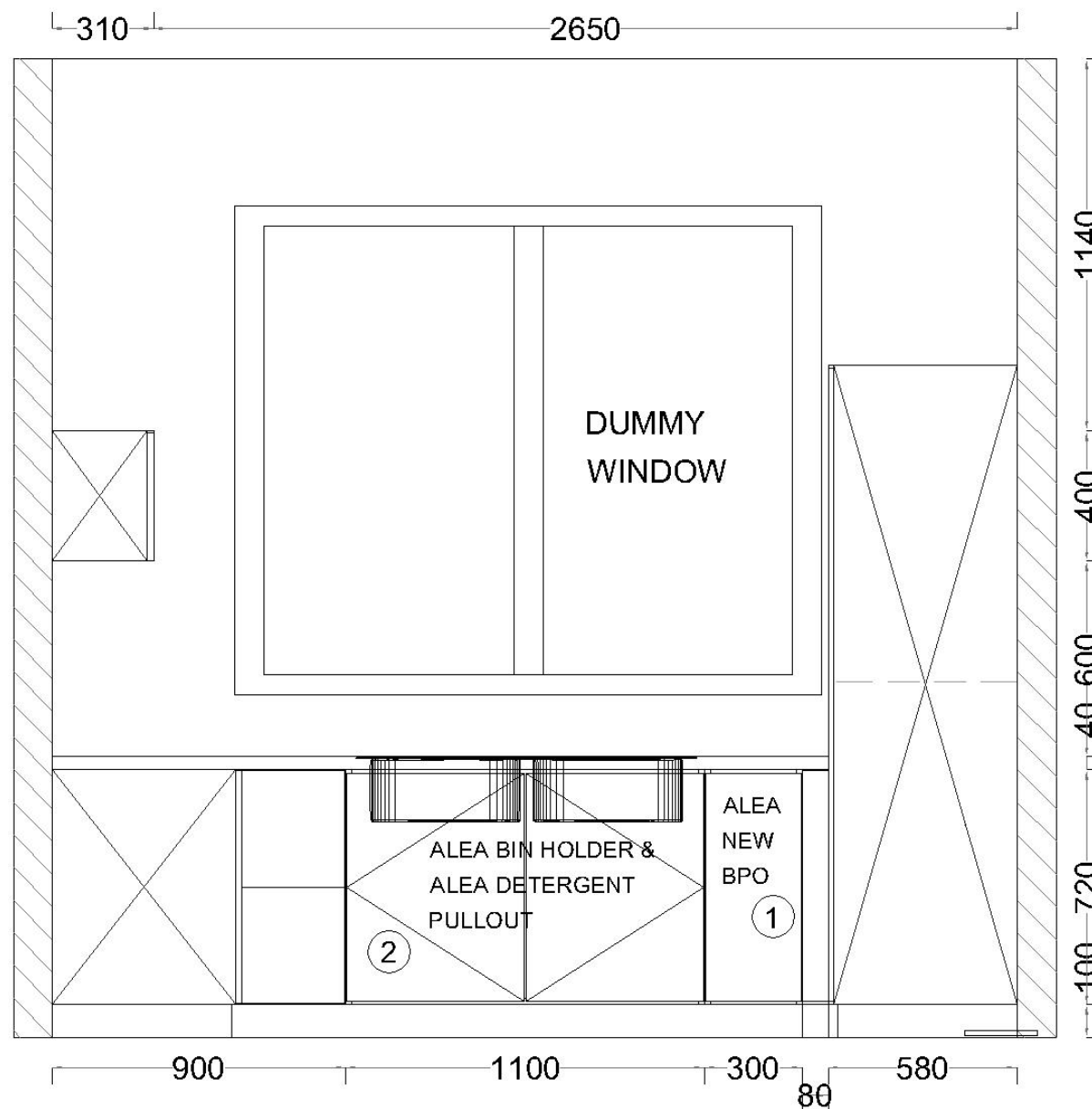
C View elevation drawing
